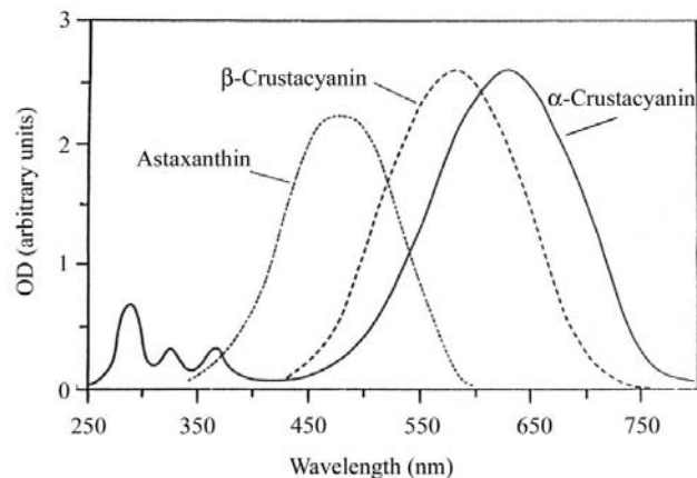
Figure 4 Absorption spectra: astaxanthin in hexane, \beta -crustacyanin, \alpha -crustacyanin.
